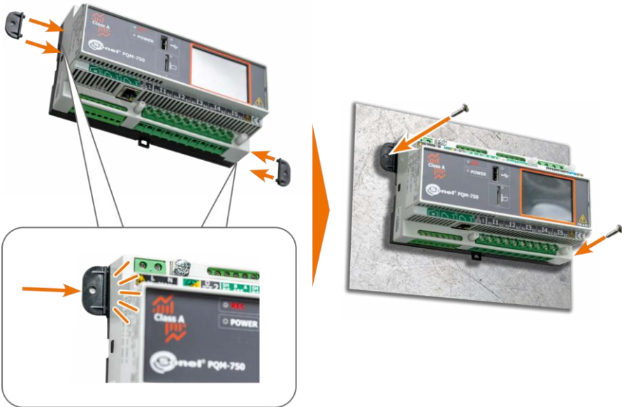
Fig. 6. Mounting the analyzer to the wall using the supplied brackets.
