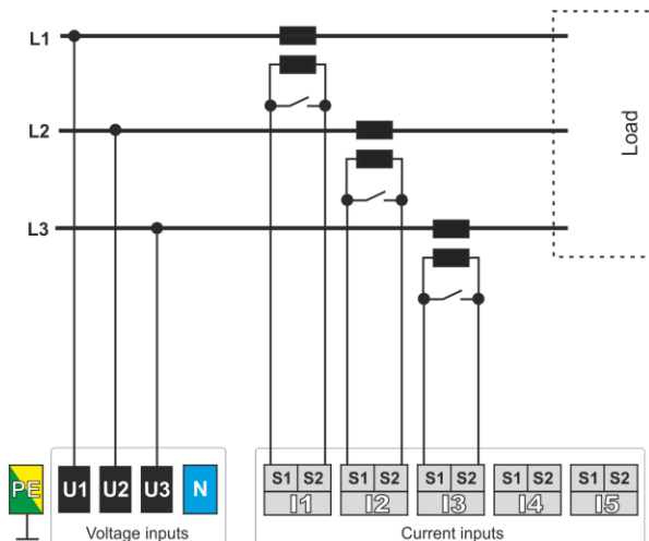
Fig. 28. Wiring diagram – 3-phase 3-wire, direct voltage connection.
