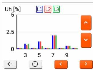
Fig. 14. Voltage harmonics screen. Nine harmonics are shown on each screen, and pressing up and down arrows allows switching to next or previous nine harmonics. Pressing right arrow switches to the current harmonics.
