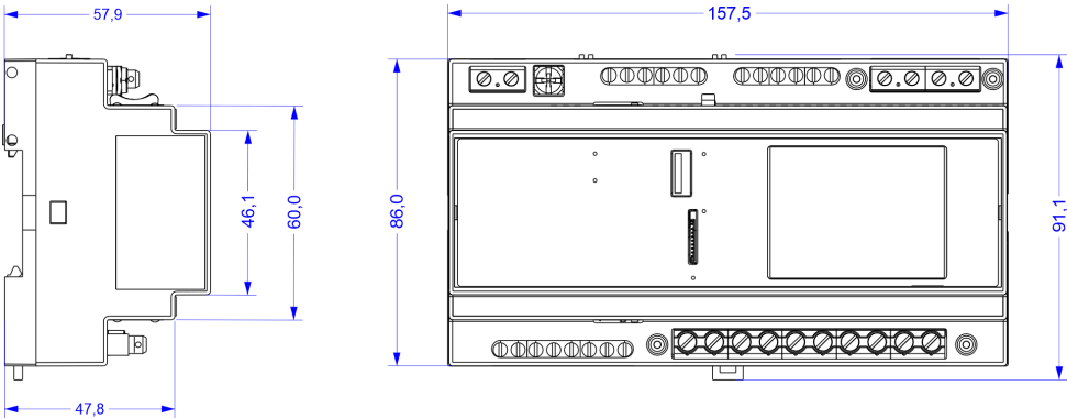
Fig. 4. Analyzer's external dimensions (in millimeters).
