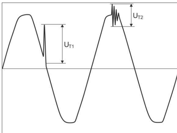
Fig. 36. Method for determining transient amplitudes.
